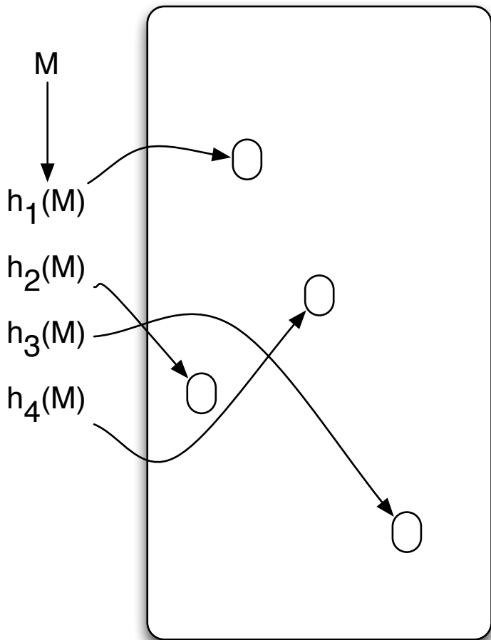
(a) Single hash table
